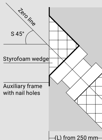
Sectional view, 45° angular double flange sleeve:
